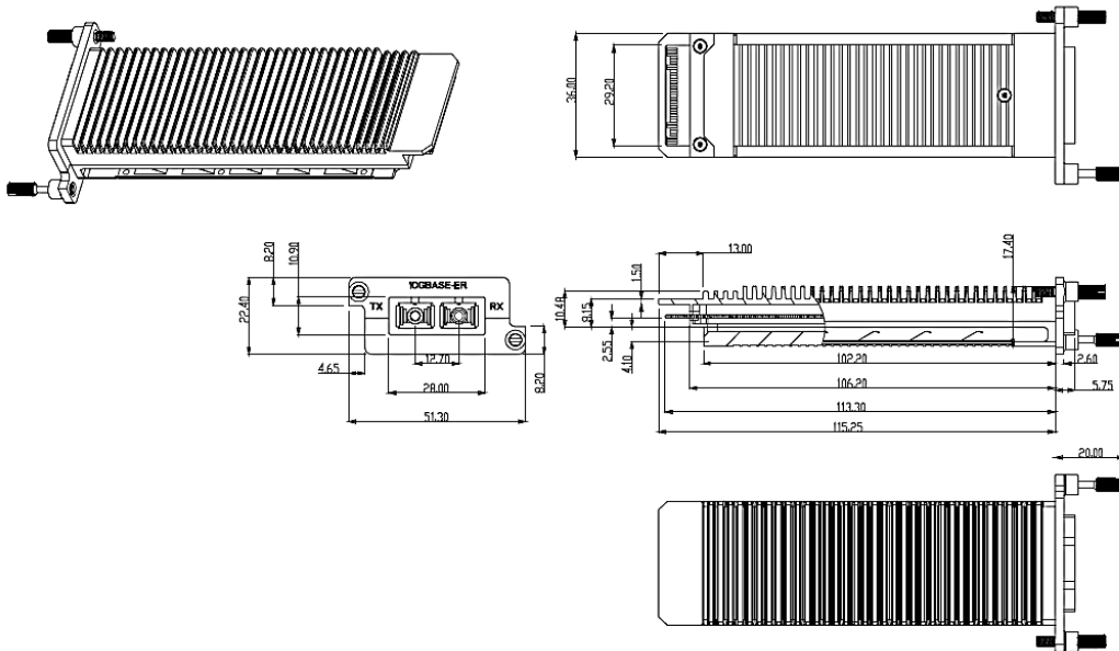
Figure 3: Mechanical Dimensions (Dimensions in mm)
