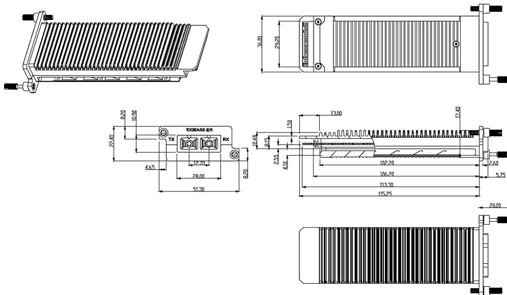
Figure 3: Mechanical Dimensions (Dimensions in mm)
