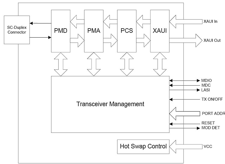
Figure 2: Functional Diagram of Typical XENPAK Style Transceiver
