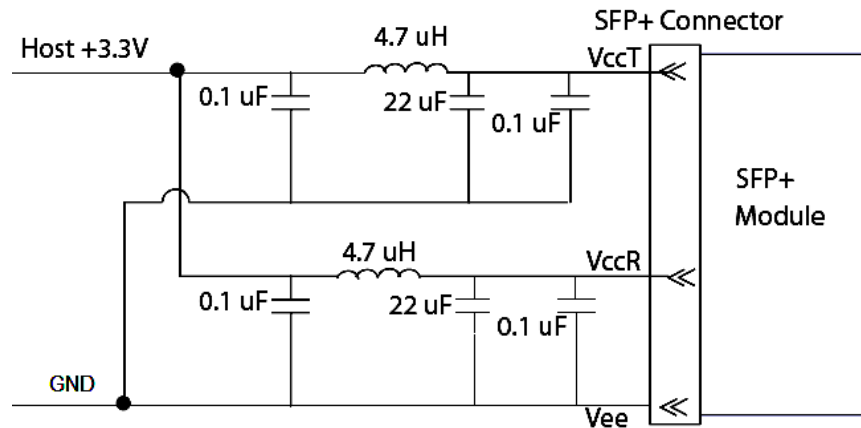
Figure2. Host Board Power Supply Filters Circuit
