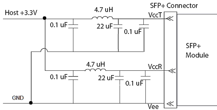
Figure3. Host Board Power Supply Filters Circuit
