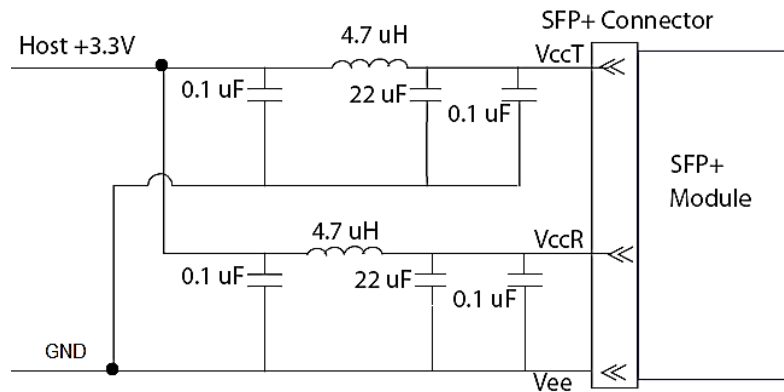
Figure3. Host Board Power Supply Filters Circuit
