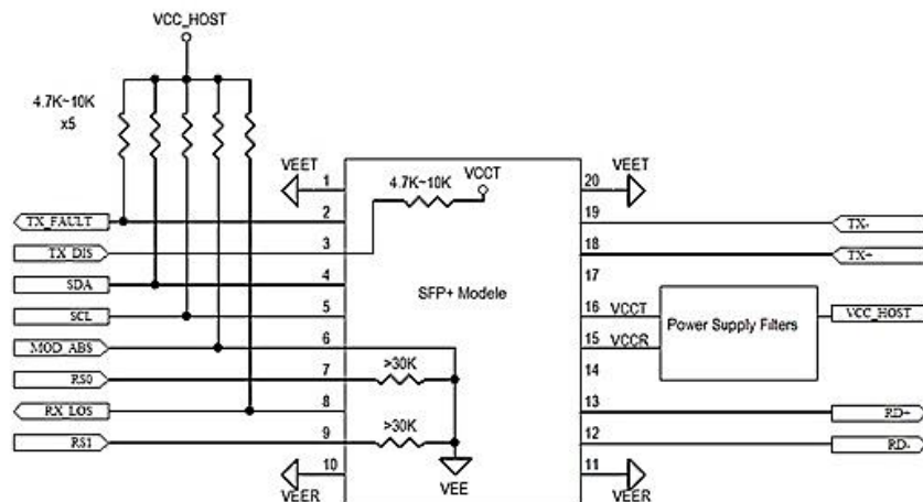
Figure3. Host Board Power Supply Filters Circuit
