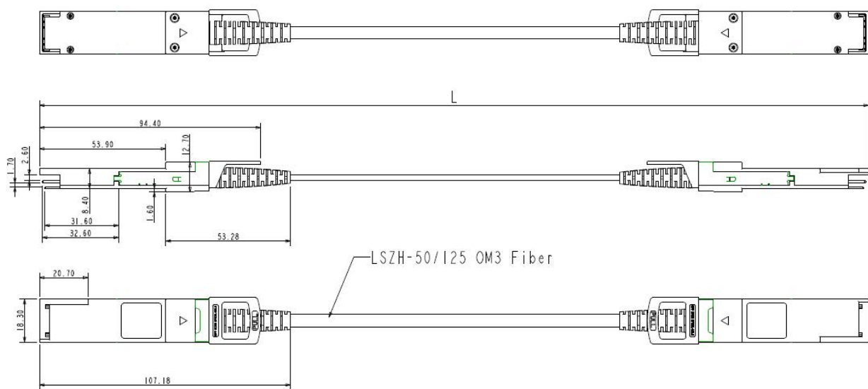
Figure2. Mechanical Specifications
